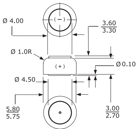
Industry Standard Dimensions (mm)
